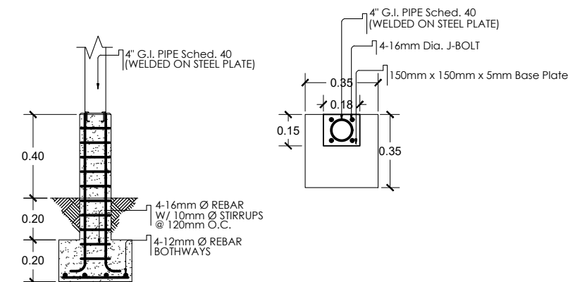
POST & FOOTING DETAIL SCALE : 1 : 25 m
