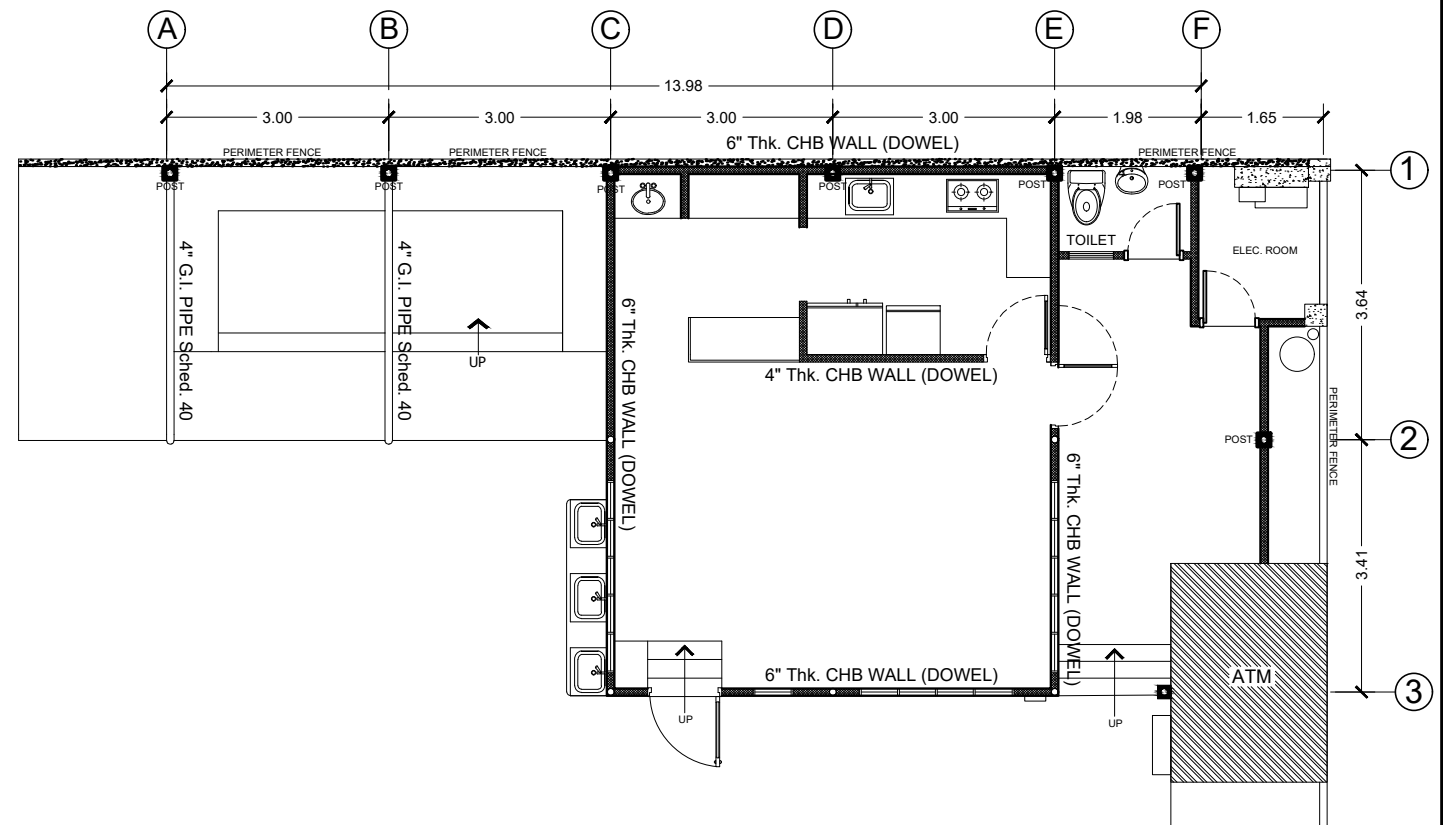
DRIVERS LOUNGE & CANTEEN FOUNDATION PLAN SCALE : 1 : 100 m
