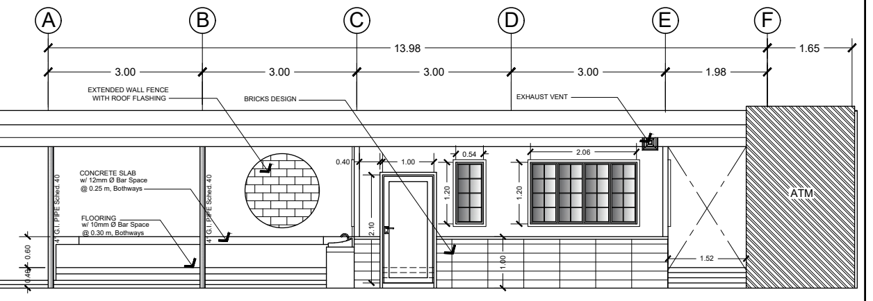
FRONT ELEVATION SCALE : 1 : 100 m
