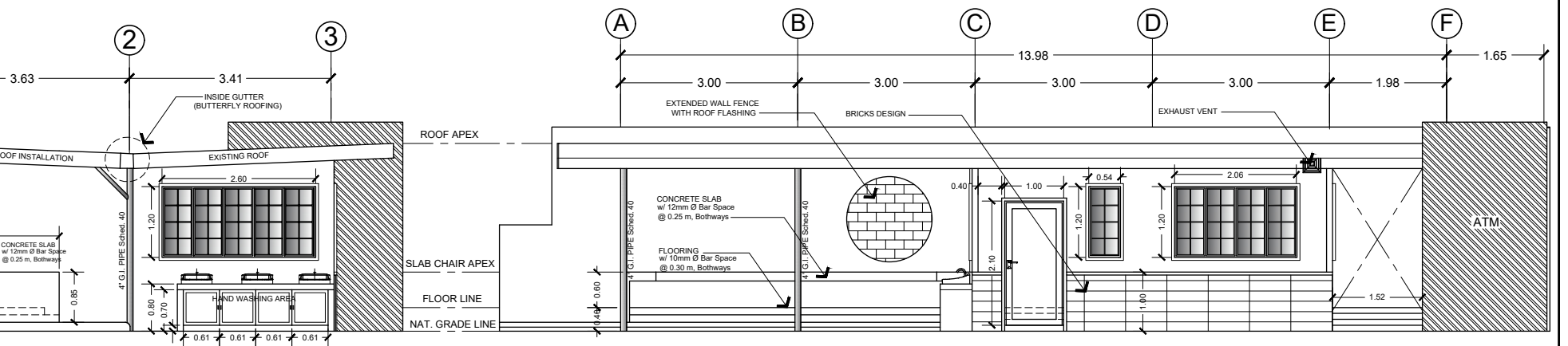
FRONT ELEVATION SCALE : 1 : 100 m
