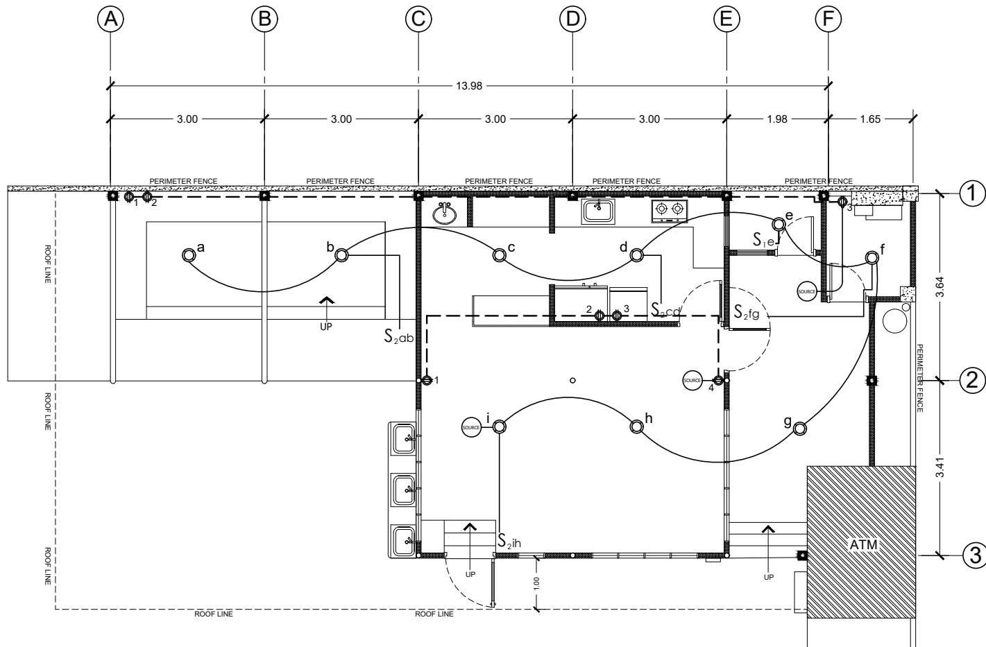
DRIVERS LOUNGE & CANTEEN ELECTRICAL PLAN SCALE : 1 : 100 m
